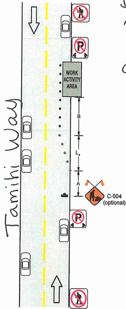
Figure 7.6: Work in Parking Lane - Urban Area
